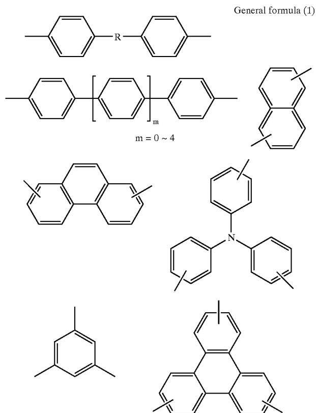
General formula (1)
