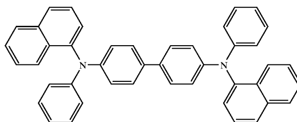
NPD
