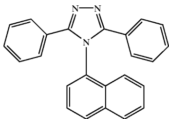
3-phenyl-4-(1-naphthyl)-5-phenyl-1,2,4-triazole
