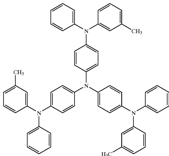
Structural formula (5)
