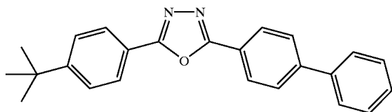
2-(4-tert-butylphenyl)-5-(4-biphenyl)-1,3,4-oxadiazole
