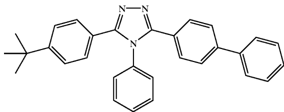
3-(4-tert-butylphenyl)-4-phenyl-5-(4'-biphenyl)-1,2,4-triazole
